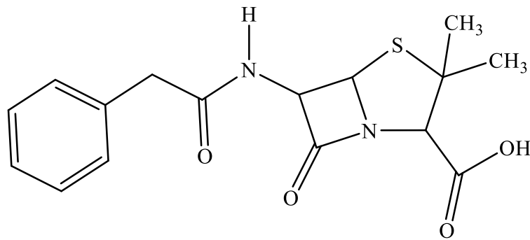
3,3-dimethyl-7-oxo-6-(2-phenylacetamido)-4-thia-1-azabicyclo[3.2.0]heptane-2-carboxylic acid (Penicillin)
