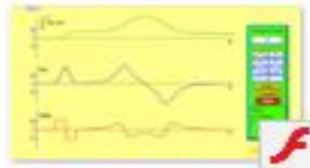
Calculus Grapher
