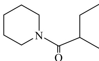
2-methyl-1-(piperidin-1-yl)butan-1-one
