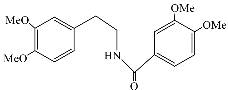
N -(3,4-dimethoxyphenethyl)-3,4-dimethoxybenzamide
