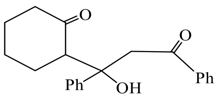
2-(1-hydroxy-3-oxo-1,3-diphenylpropyl)cyclohexan-1-one
