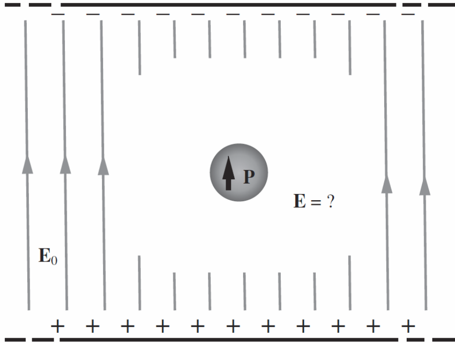
Fig. The sources of the field \mathbf{E}_0 remain fixed. The dielectric sphere develops some polarization \mathbf{P} . The total field \mathbf{E} is the superposition of \mathbf{E}_0 and the field of this polarized sphere.
