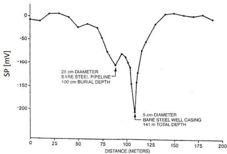
SP anomalies generated by buried metal pipelines and well casings at Meso, California, USA
