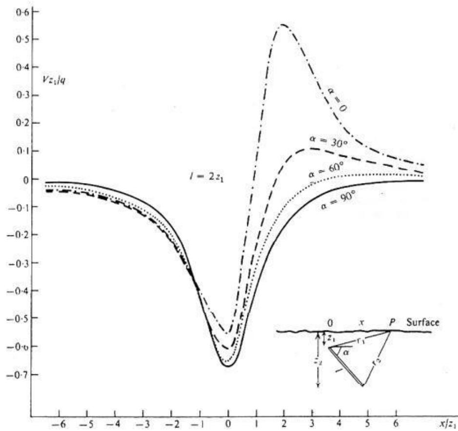
SP profiles over buried polarized rod
