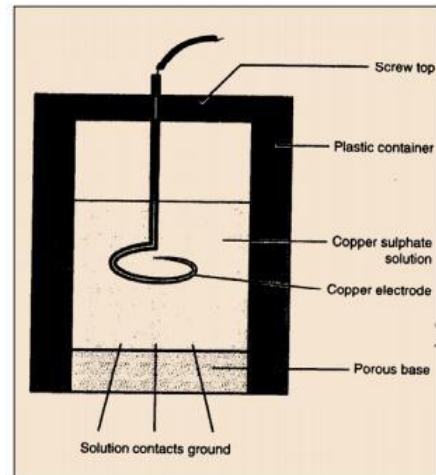
Porous pot electrodes
